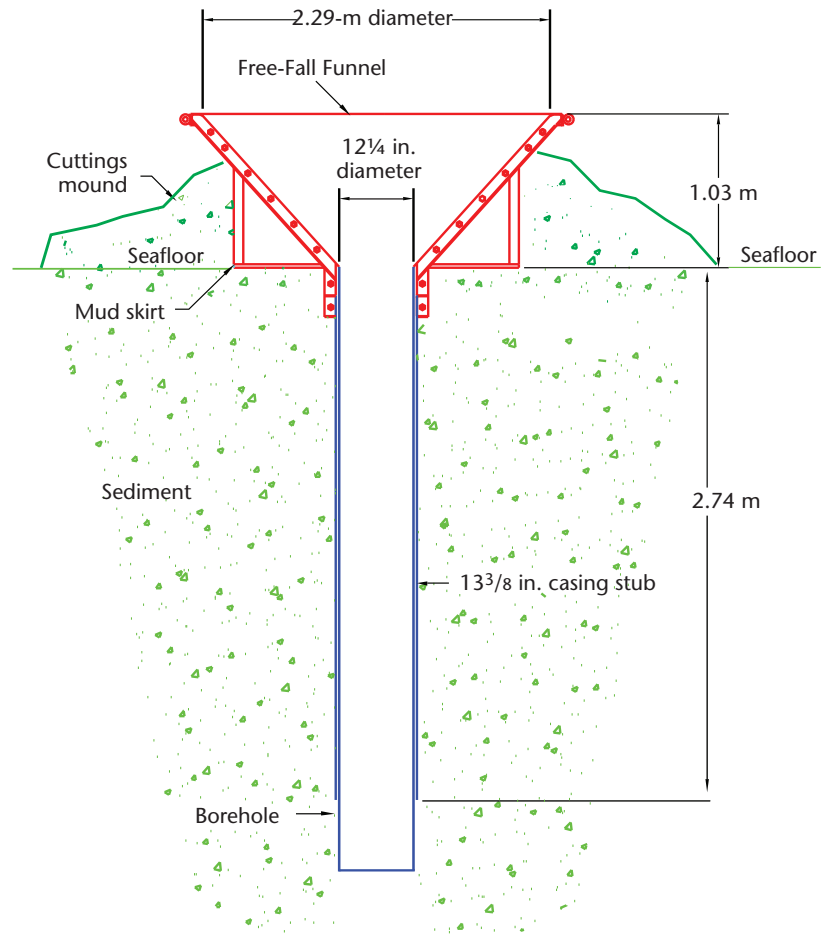
Schematic of the FFF deployed in sediment. After a hole is drilled in sediment, a FFF can be installed to assist in reentry.
