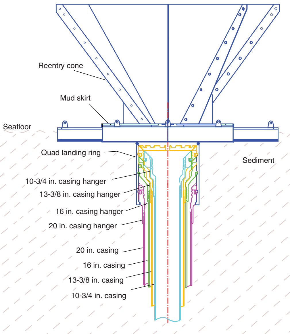
Schematic of the reentry cone, mud skirt, and housing with four Drill-Quip casing hangers (20 in., 16 in., 13 3 / 8 in., 10 3 / 4 in.) landed in the housing.
